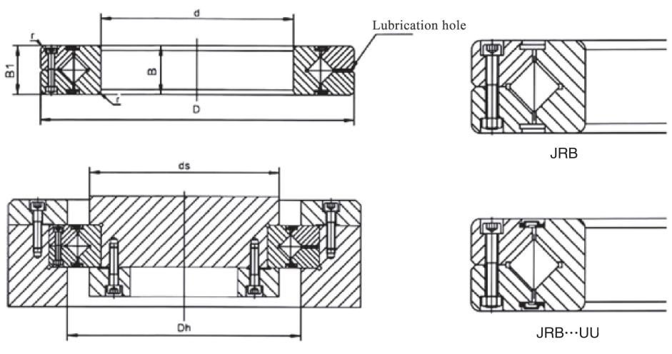
Separable outer ring, overall inner ring
